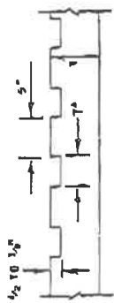
ALTERNATE SECTION B-B (SAMED RUMBLE STRIP) RUMBLE STRIP FOR HOT MIX ASPHALT SHOULDERS
