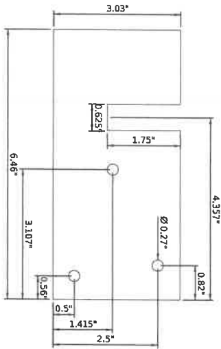
STEEL DECK CLIP FOR 5/8" FLANGE
