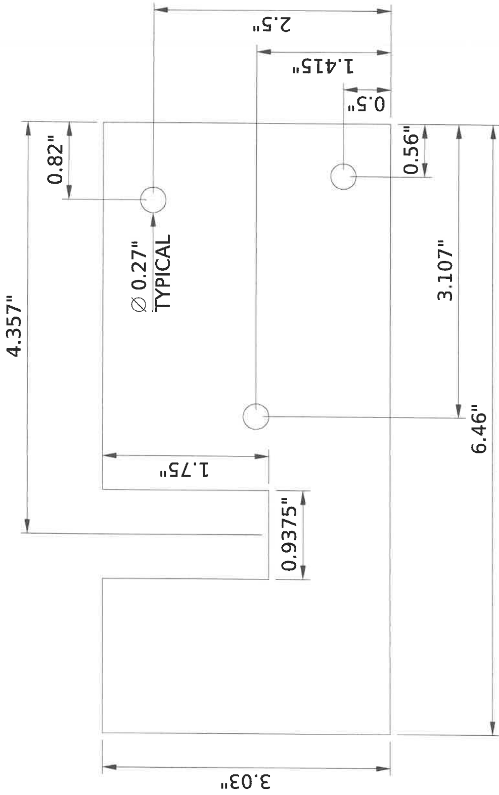
STEEL DECK CLIP FOR 15/16" FLANGE
