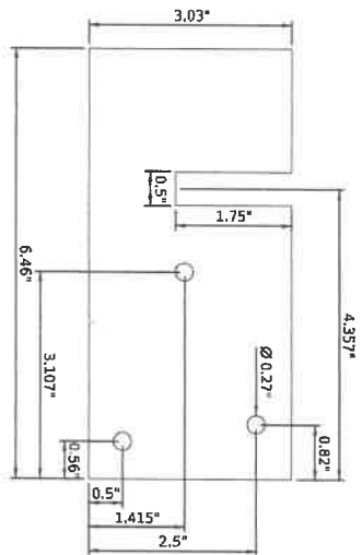
STEEL DECK CLIP FOR 1/2" FLANGE
