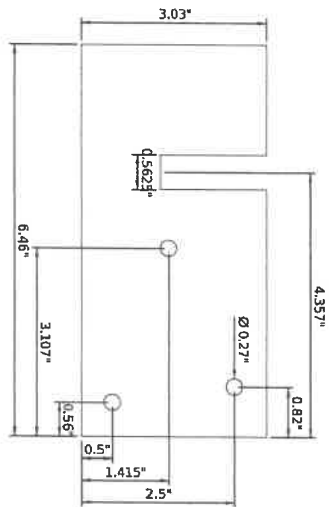
STEEL DECK CLIP FOR 9/16" FLANGE
