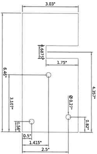
STEEL DECK CLIP FOR 11/16" FLANGE
