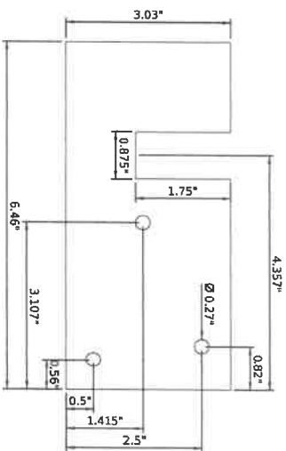
STEEL DECK CLIP FOR 7/8" FLANGE
