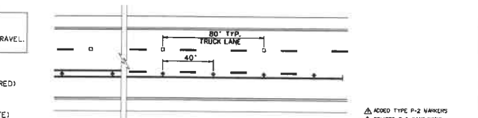
TWO LANE HIGHWAY WITH TRUCK CLIMBING LANE
