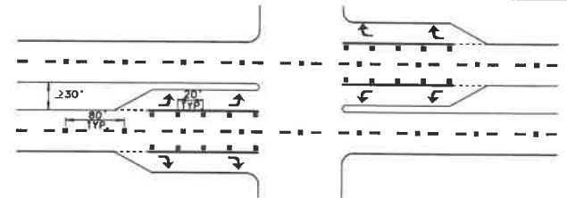
MULTI-LANE ROADWAY WITH AT-GRADE INTERSECTION
