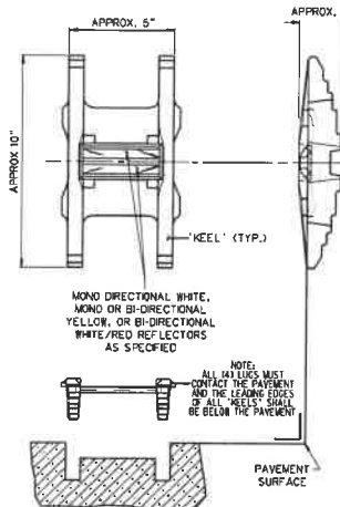
TYPICAL TYPE "P-2" MARKER (ITEM 663012-*)
