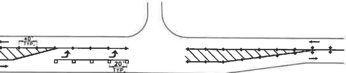
TWO LANE HIGHWAY WITH LEFT TURN BAY
