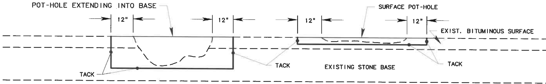
(ELEVATION VIEW)
