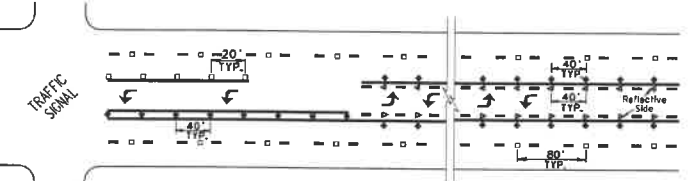
MULTI-LANE ROADWAY WITH TWO-WAY LEFT TURN LANE
