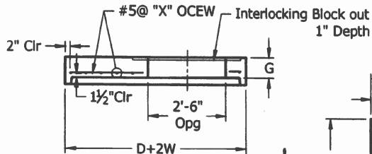
Section View
