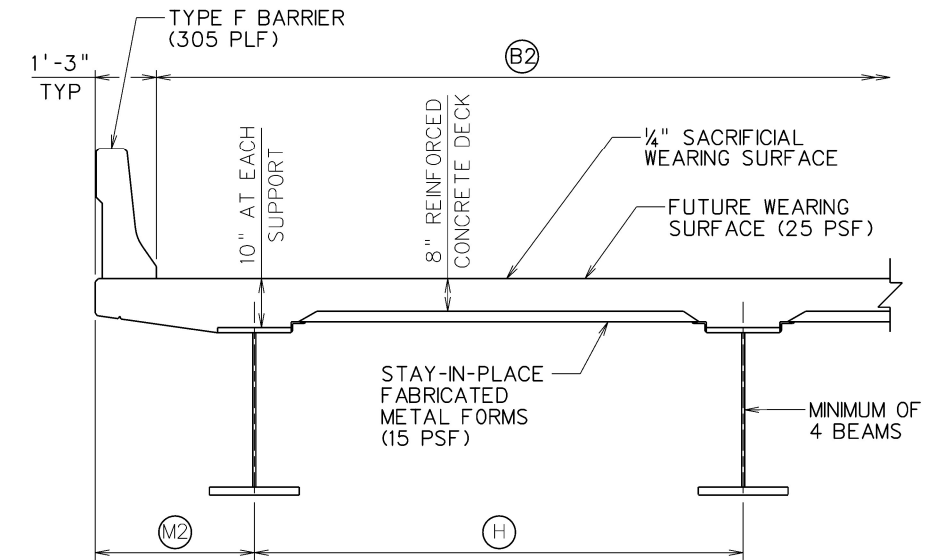
PARTIAL TYPICAL SECTION
