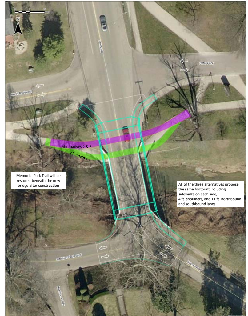
Alternative 2 Two Span Concrete Hybrid I-Beam $1,839,500*
