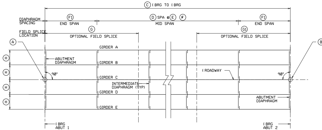
FRAMING PLAN
