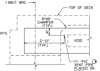
VENT PIPE DETAIL (TYPICAL EACH END)
