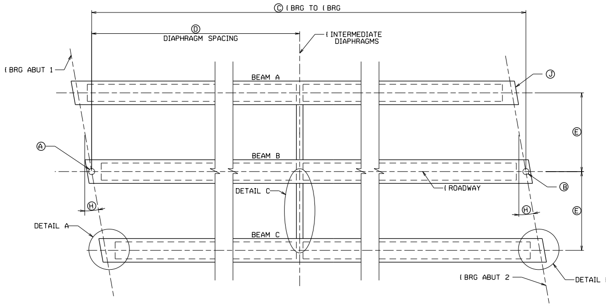
FRAMING PLAN
