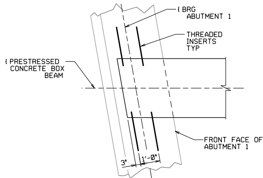
DETAIL A (TYP) ABUTMENT 1
