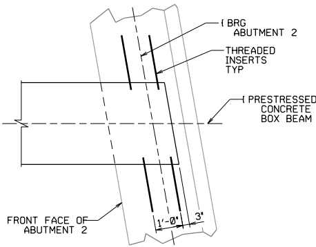
DETAIL B (TYP) ABUTMENT 2
