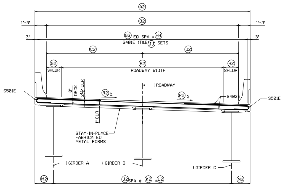
TYPICAL SECTION LOOKING STATION AHEAD
