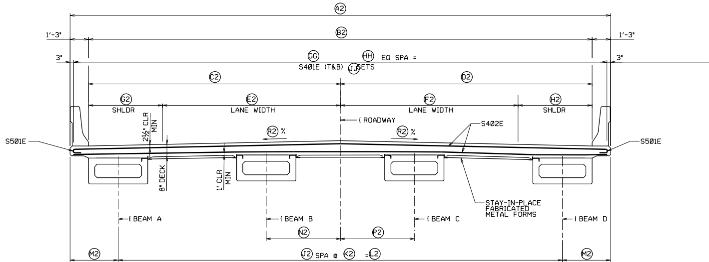
TYPICAL SECTION LOOKING STATION AHEAD
