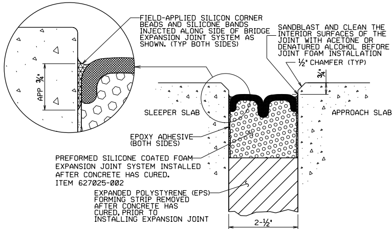
EXPANSION JOINT SEALING DETAIL (FOR MOVEMENTS 2 1/4')
