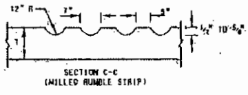
MILLED RUMBLE STRIP FOR PORTLAND CEMENT AND HOT MIX ASPHALT SHOULDERS
