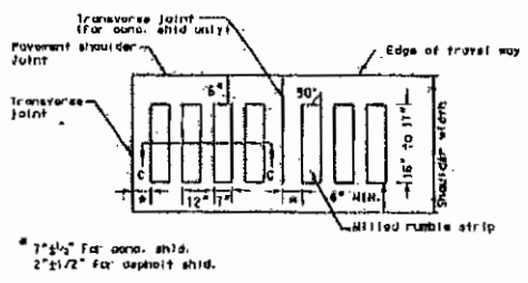
MILLED RUMBLE STRIP FOR PORTLAND CEMENT AND HOT MIX ASPHALT SHOULDERS
