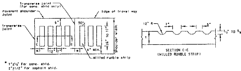
MILLED RUMBLE STRIP FOR PORTLAND CEMENT AND HOT MIX ASPHALT SHOULDERS
