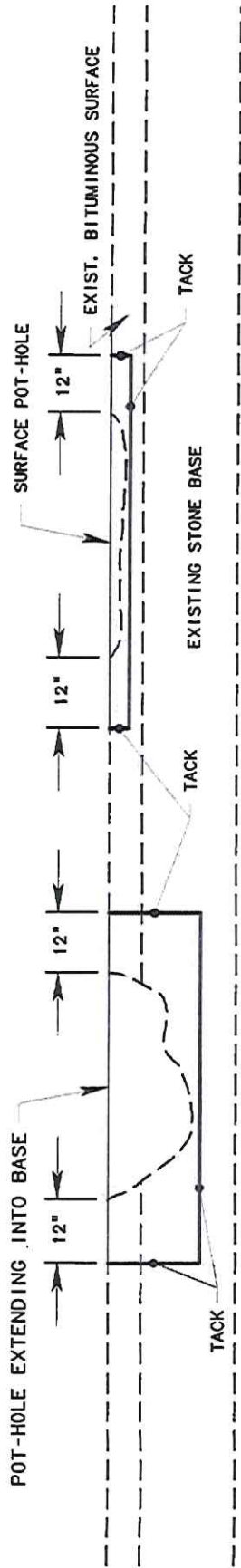
(ELEVATION VIEW)
