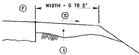
NORMAL SECTIONS
