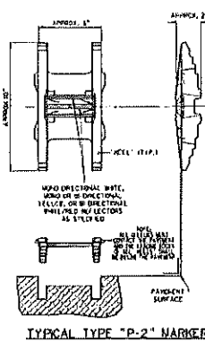
TYPICAL TYPE "P-2" MARKER ITEM 85302-02
