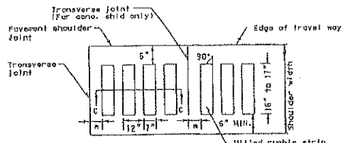
MILLED RUMBLE STRIP FOR PORTLAND CEMENT AND HOT MIX ASPHALT SHOULDERS
