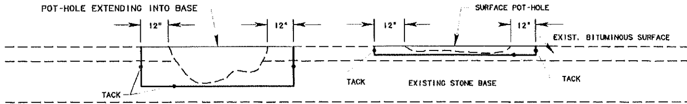
(ELEVATION VIEW)
