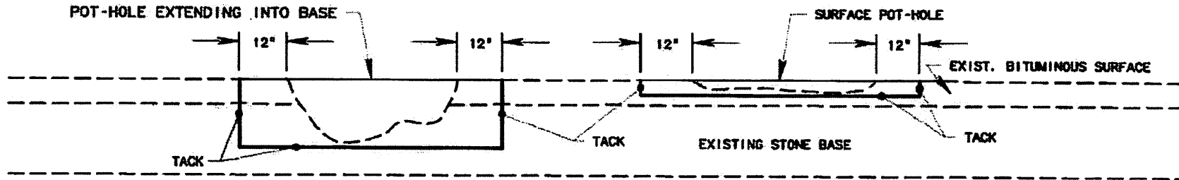
(ELEVATION VIEW)
