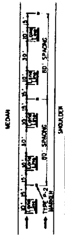
LANE LINE OF DIVIDED HIGHWAY
