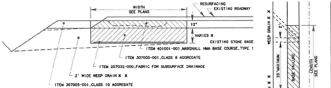
(ELEVATION VIEW)
