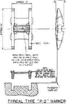
TYPICAL TYPE 'P-2' MARKER ITEM 502002-01
