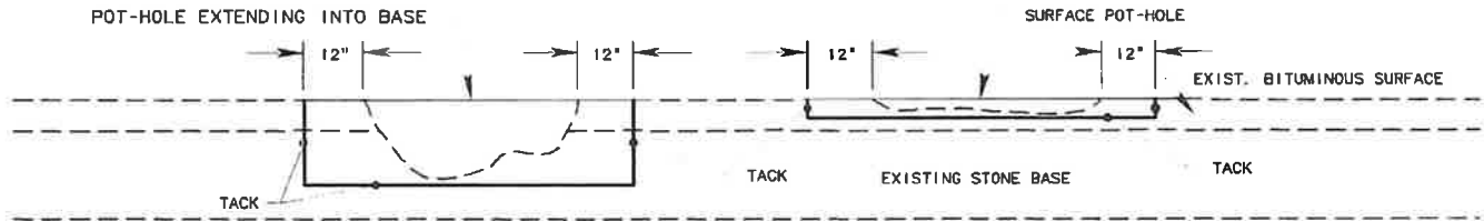
(ELEVATION VIEW)
