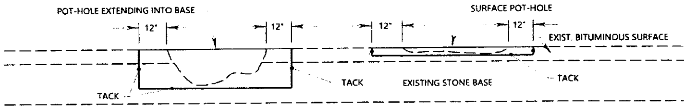
(ELEVATION VIEW)
