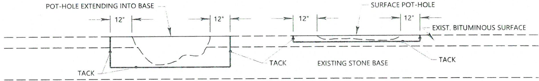
(ELEVATION VIEW)
