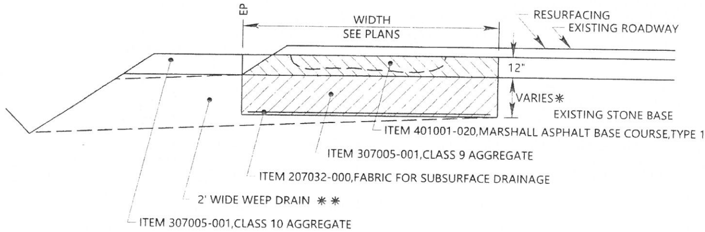
(ELEVATION VIEW)
