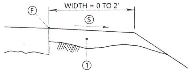
NORMAL SECTIONS
