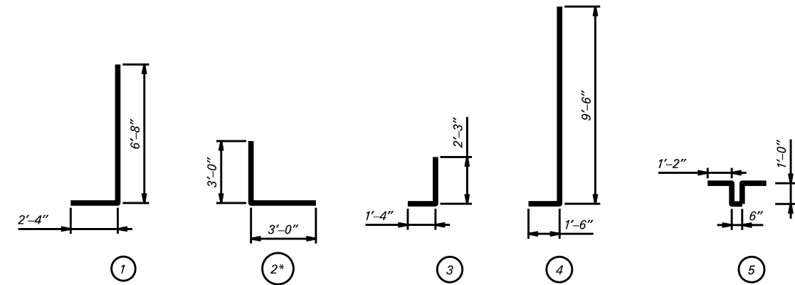
BENT REBAR DETAIL
