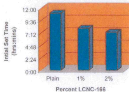
Setting Time: Plain Vs. LCNC-166
