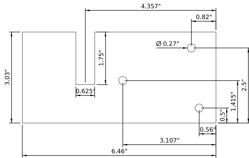
STEEL DECK CLIP FOR 5/8" FLANGE
