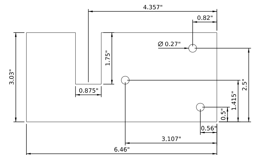
STEEL DECK CLIP FOR 7/8" FLANGE
