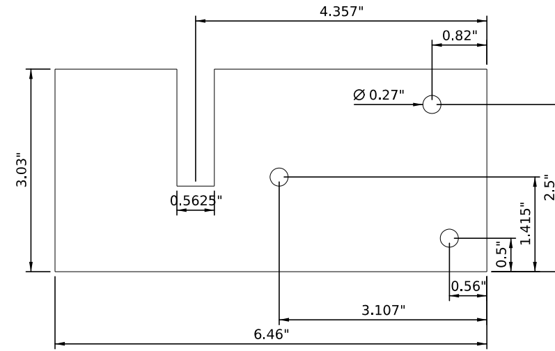
STEEL DECK CLIP FOR 9/16" FLANGE
