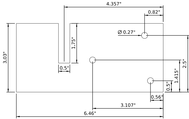
STEEL DECK CLIP FOR 1/2" FLANGE
