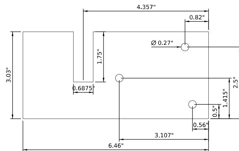
STEEL DECK CLIP FOR 11/16" FLANGE
