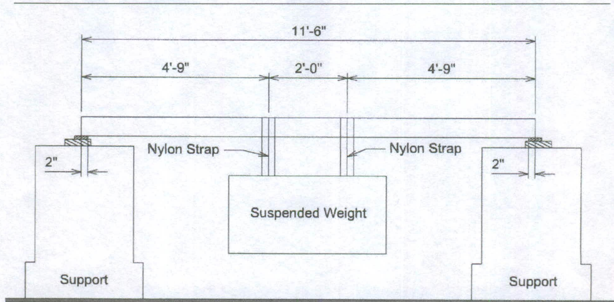
Figure 2. Test Setup
