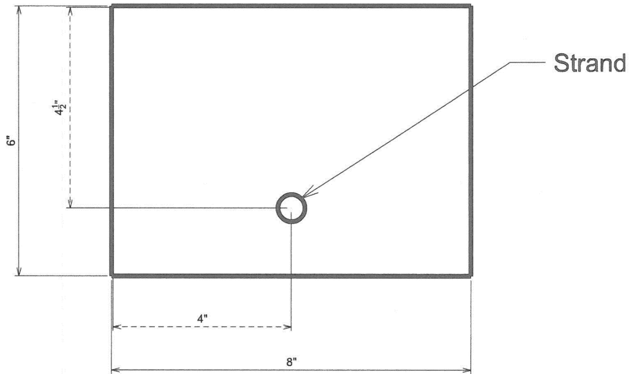
Figure 1. This drawing shows a cross section of the quality assurance test beam. (1 in = 25.4 mm) Dimensional tolerance: \pm 1/8 inch
