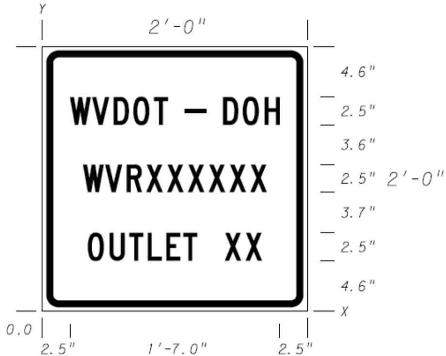
Figure 638.6.1: Outlet Marker
