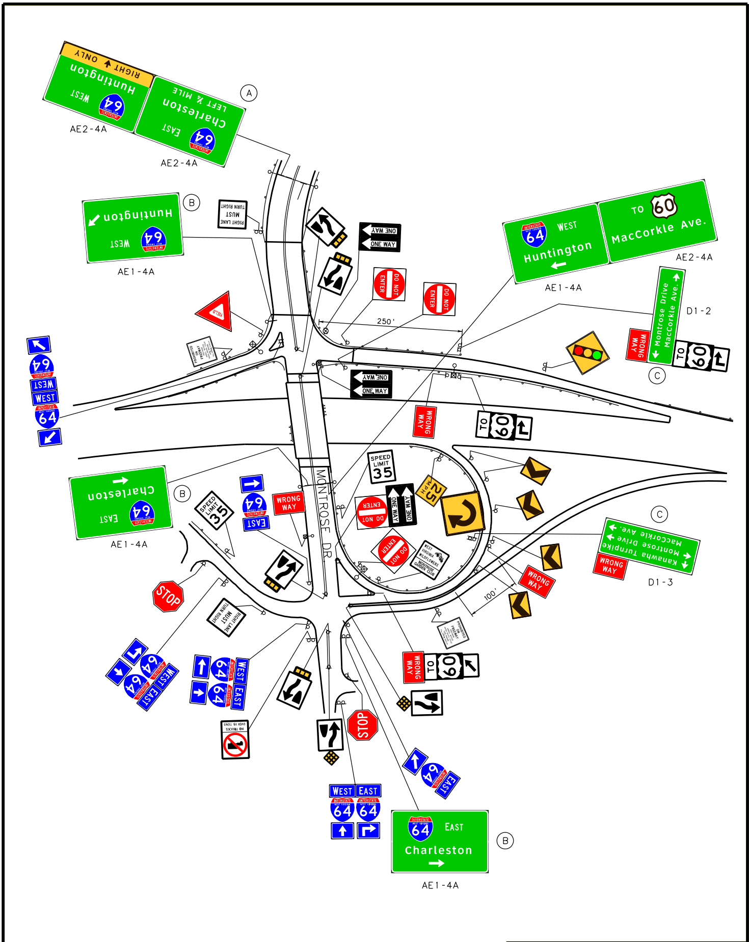
FIGURE 7 REGULATORY & WARNING SIGNING WITHIN A MAJOR OR INTERMEDIATE INTERCHANGE
