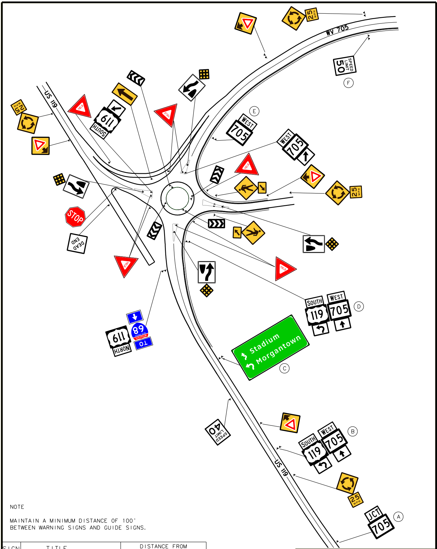
FIGURE 11B SIGNING FOR MULTI-LANE ROUNDABOUT
