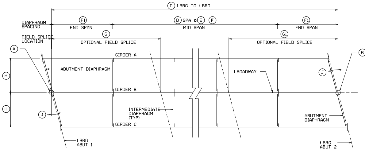
FRAMING PLAN
