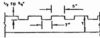
ALTERNATE SECTION 0-0 (SAVED RUMBLE STRIP) RUMBLE STRIP FOR HOT MIX ASPHALT SHOULDERS
