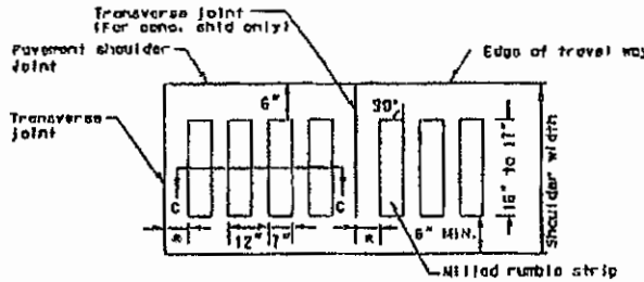
MILLED RUMBLE STRIP FOR PORTLAND CEMENT AND HOT MIX ASPHALT SHOULDERS
