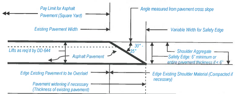
Safety Edge Dimensions for Asphalt Pavement (Overlay – for Roadways with Established Design Criteria, i.e. Interstate, APD, NHS and US Routes)
