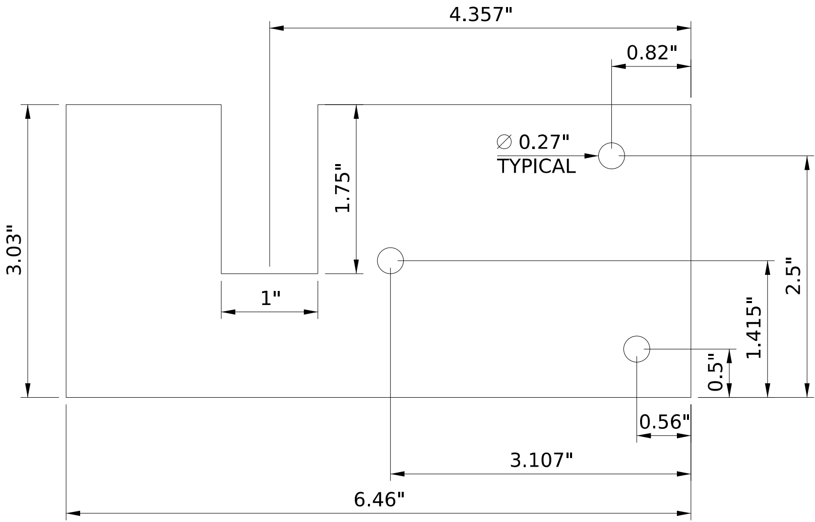
STEEL DECK CLIP FOR 1" FLANGE
