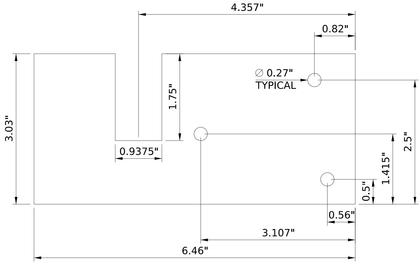
STEEL DECK CLIP FOR 15/16" FLANGE
