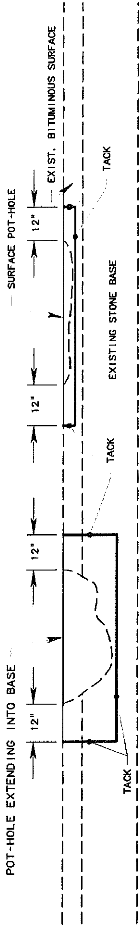
(ELEVATION VIEW)
