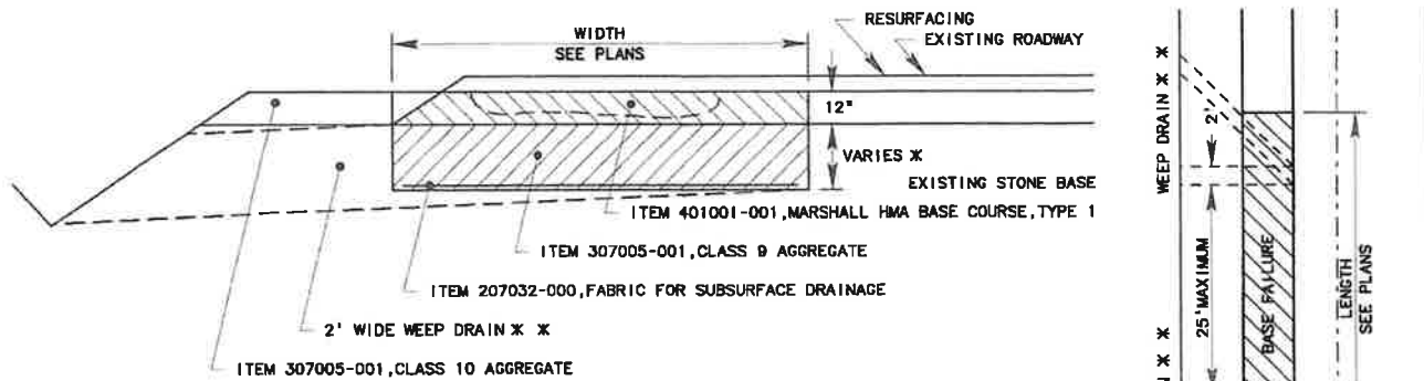
(ELEVATION VIEW)
