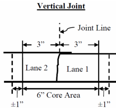
Figure 1 – Cross-sectional View, Position of Core Along Longitudinal Joint, Imperial Units
